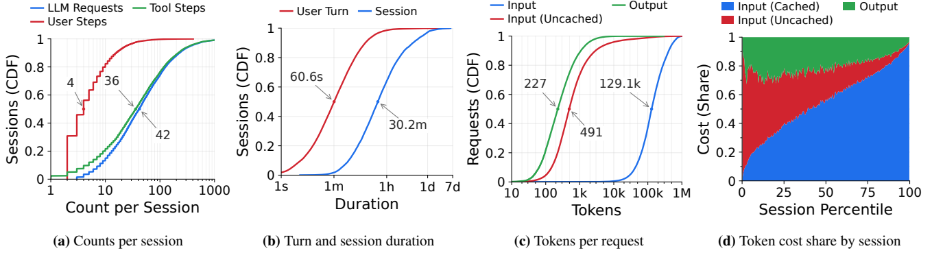
Figure 2: (a) Sessions contain a few user steps but tens to hundreds of LLM requests, most of them triggered by tools. (b) A single user turn lasts from a few seconds to more than 24 hours, while a typical session lasts from a few minutes to almost one week. (c) Requests carry long inputs, with most tokens being cached. (d) The cost of most sessions is dominated by prefix-cache hits.
