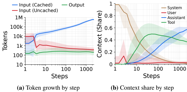
Figure 3: Context composition changes as a session progresses. Shaded areas show the P25–P75 ranges. (a) Cached tokens accumulate rapidly across steps, while uncached input and output remain small. (b) Earlier turns are dominated by the system prompt, middle turns are dominated by tool results, and later turns are dominated by LLM responses.
