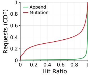
Figure 9: Context mutations break reuse: the hit ratio on the step after a mutation is far below the step after an append.
