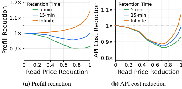
Figure 12: Lowering cache-read prices to reduce context mutations does not necessarily reduce prefill or API cost as contexts become longer and misses become more expensive. We assume harnesses reduce mutations linearly as cache reads become cheaper, varying retention times and compare against today’s repriced token volume.
