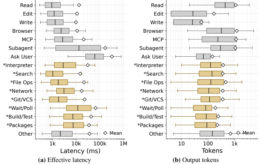
Figure 5: Tool categories differ substantially in both latency and output size. Boxes show the P5–P95 range, and diamonds denote the mean. (a) Effective tool-execution latency. (b) Number of tokens added to the context by tool execution.
