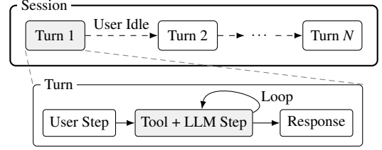
Figure 1: Coding-agent execution hierarchy. A session is a sequence of user turns separated by user idle time. Each turn begins with a user step, and continues through a repeated LLM–tool loop.
