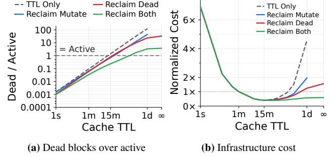
Figure 13: Session-level signals reclaim dead blocks invalidated by context mutations or left behind by completed sessions before their TTL expires. Reclaiming both sources helps on both counts in simulation. (a) Dead blocks fall by about 36\times at a one-day TTL. (b) Infrastructure cost stays low even at long TTLs.
