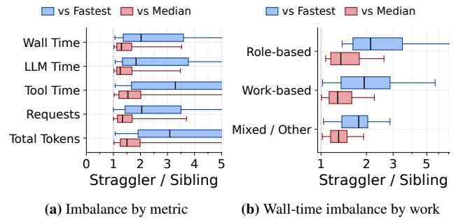
Figure 7: Straggler imbalance in synchronous subagent fan-out. (a) The slowest sibling is typically about 2\times slower than the fastest, with the largest gap in tool time. (b) Role-based fan-outs exhibit greater wall-time imbalance than work-based and mixed fan-outs.
