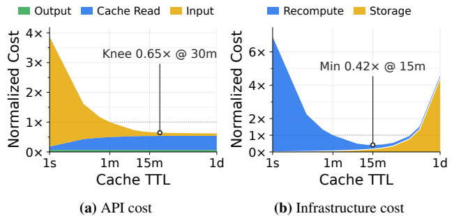
Figure 11: Longer retention reduces API cost by avoiding recomputation. Cost is normalized to a 1-minute TTL. (a) Most savings are captured within 30 minutes, at 0.65 \times . (b) Infrastructure cost reaches its minimum of 0.42 \times at 15 minutes, after which the added storage overhead outweighs further recomputation savings.
