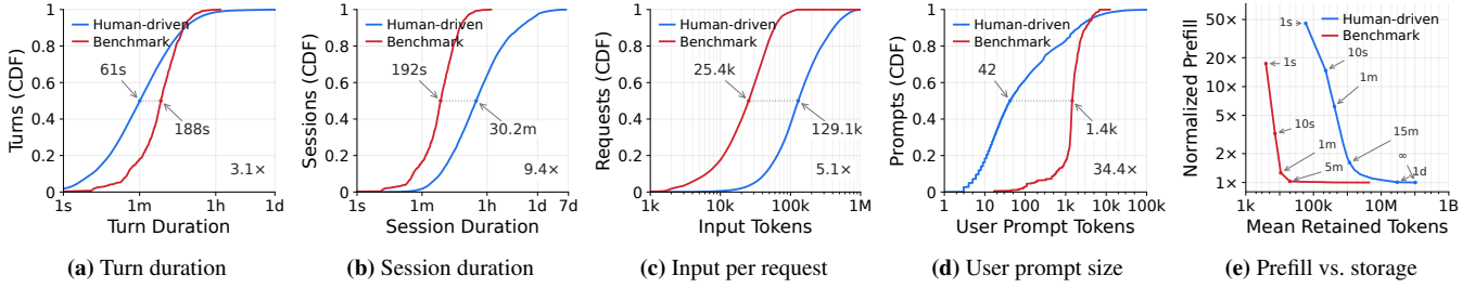
Figure 14: Benchmark replay and production sessions stress serving systems differently. (a) SWE-Bench has longer uninterrupted single-turn execution. (b) Production sessions span multiple turns and last longer overall. (c) Production sessions accumulate larger contexts. (d) SWE-Bench prompts are longer and more uniform, whereas production prompts are shorter and more variable. (e) Five minutes of retention brings SWE-Bench prefill within 3% of its infinite-retention floor; production first reaches this range at one day among the evaluated TTLs.
