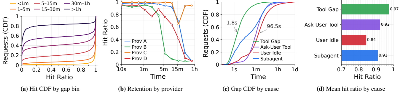
Figure 8: Prefix reuse falls as inter-request gaps grow. (a) Short gaps preserve most of the cached prefix, while longer gaps are associated with more misses. (b) Prefix retention varies across providers, ranging from minutes to beyond an hour. (c) Ordinary tool gaps are typically short, while user idle time, Ask User tools, and subagent execution introduce longer gaps. (d) Cache loss is more common after these longer gaps.
