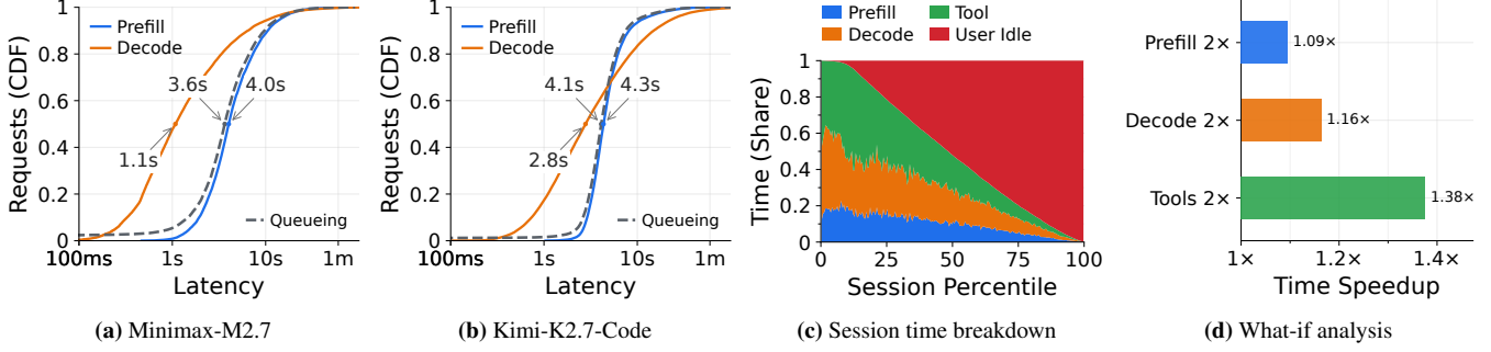
Figure 4: Request and session latency have different bottlenecks. Request latency is strongly shaped by TTFT serving overheads. (a, b) For externally routed models like Minimax-M2.7 and Kimi-K2.7-Code, TTFT is dominated by these overheads rather than pure prefill. (c) At the session level, tool execution and user idle time account for much of the session time. (d) With user idle time excluded and each tool gap capped at 15 minutes, accelerating tools yields larger gains than accelerating prefill or decode.
