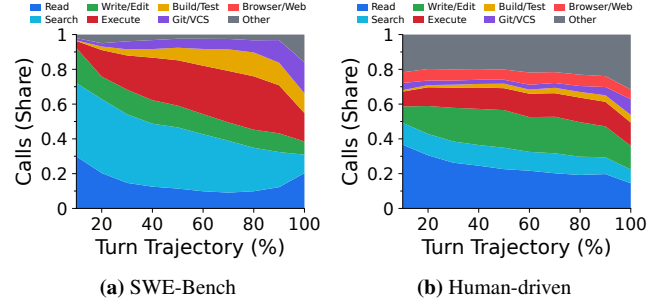
Figure 15: Tool usage evolves differently in benchmark and human-driven turn trajectories. (a) SWE-Bench shifts from Read/Search early to Execute and Build/Test later. (b) The tool mix remains more diverse throughout the turn.
