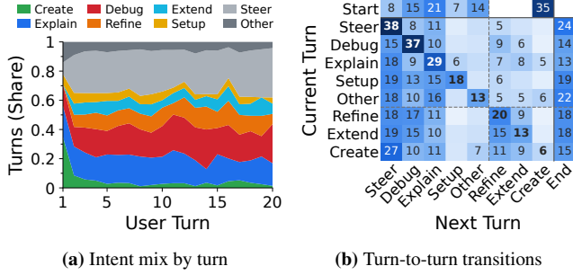
Figure 16: User prompts shift from establishing tasks to guiding execution as sessions progress. (a) Opening turns are dominated by feature-creation requests, while later turns contain more steering requests. (b) User intent also exhibits phased transitions.
