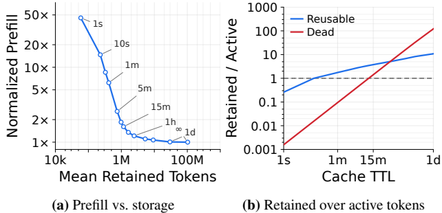
Figure 10: Longer retention reduces prefill but increases storage overhead. (a) New prefill remains 60.9% above the floor at 15 minutes, and about 1% above at one day. (b) Reusable blocks grow slowly with TTL, while dead blocks dominate at long retention and reach about 120 \times the active blocks at one day.
