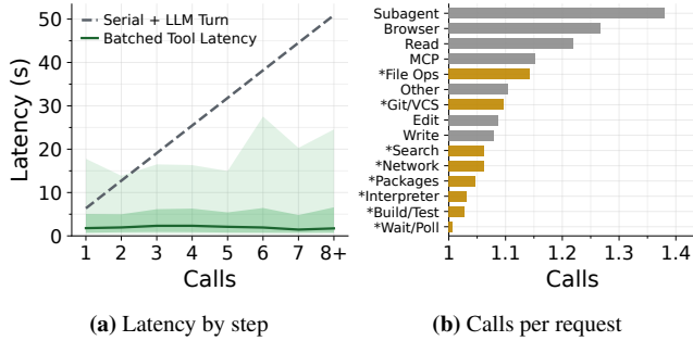
Figure 6: (a) Serial latency grows with the number of calls, while batched latency remains nearly flat. (b) Subagent, Browser, and Read are batched most frequently.
